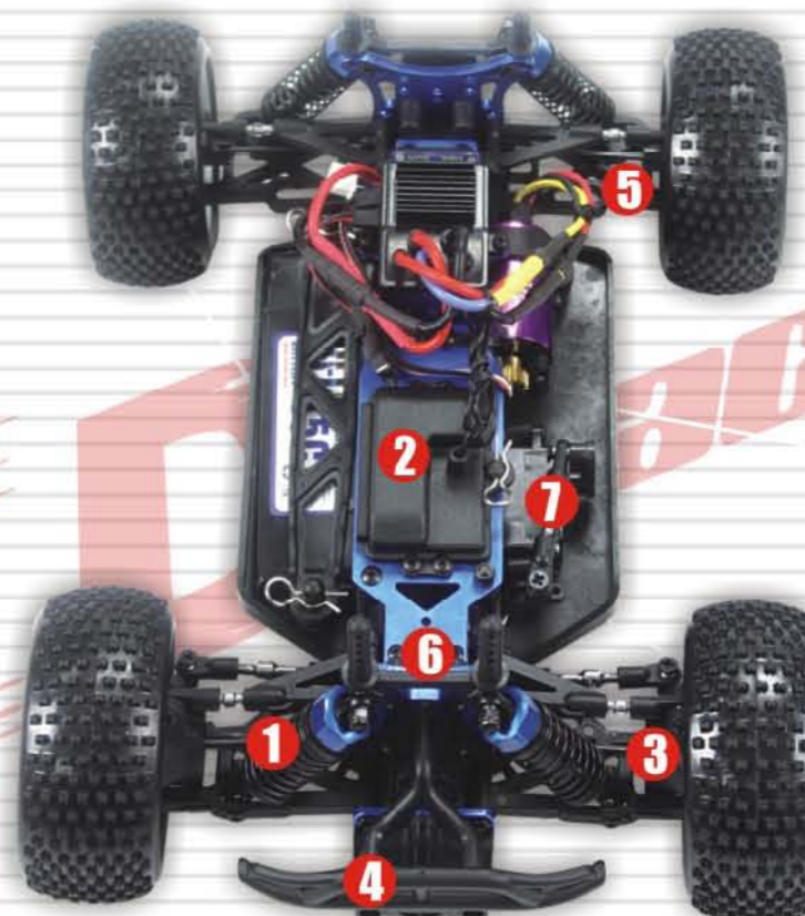
• Four wheel independent suspension, with oil filled shocks for better stability and handling
